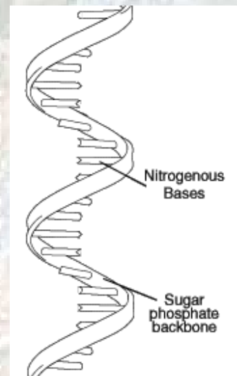
Fig. 24.3 RNA
